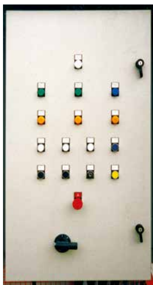
Local cabinet with motor control gear
