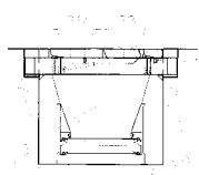
Steep Samson® Material Feeder sides plates eliminate bridging
